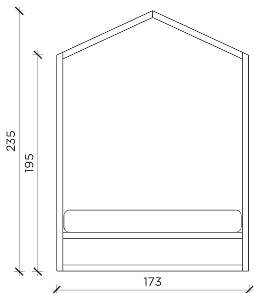
FRONTE | FRONT
