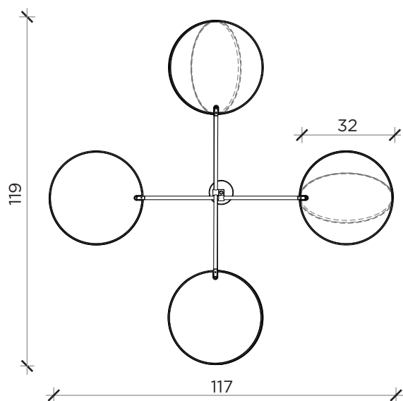
FRONTE | FRONT
