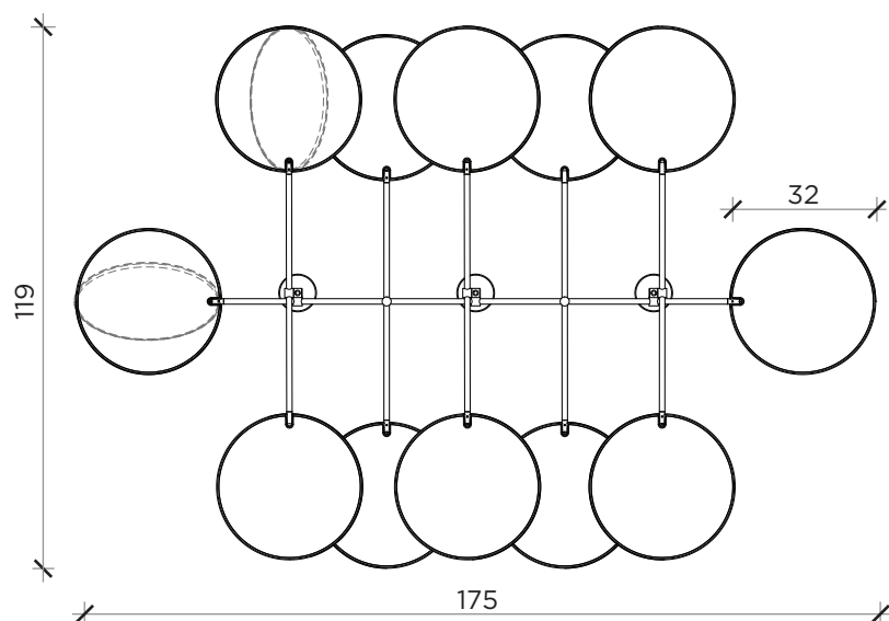
FRONTE | FRONT
