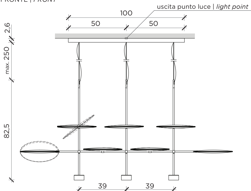
FRONTE | FRONT
