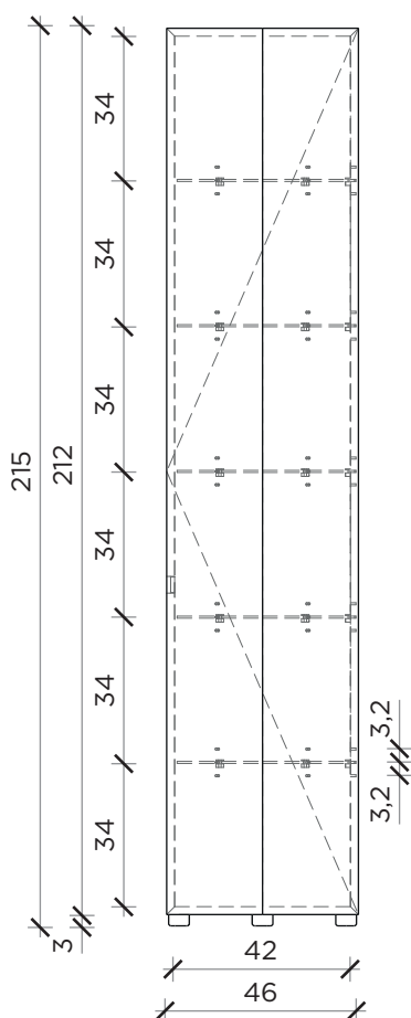
FRONTE | FRONT
