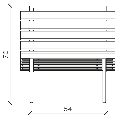
FRONTE | FRONT
