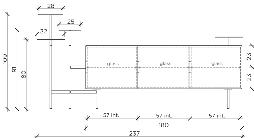
FRONTE | FRONT
