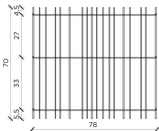
FRONTE | FRONT
