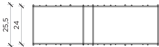
FRONTE | FRONT
