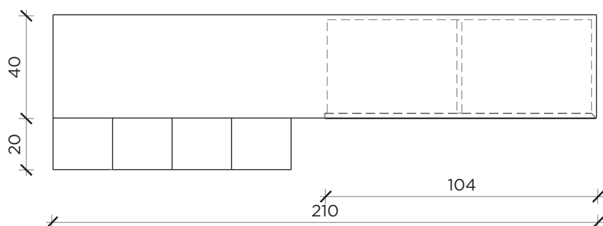
FRONTE | FRONT
