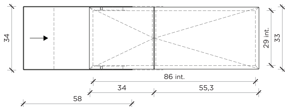
FRONTE | FRONT
