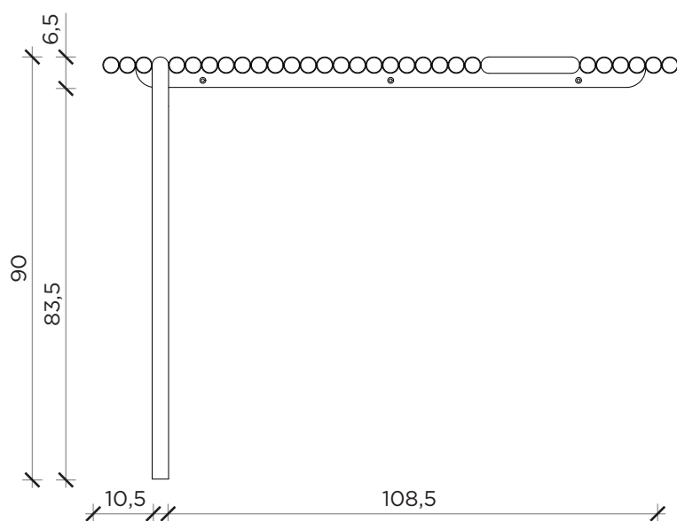
FRONTE | FRONT
