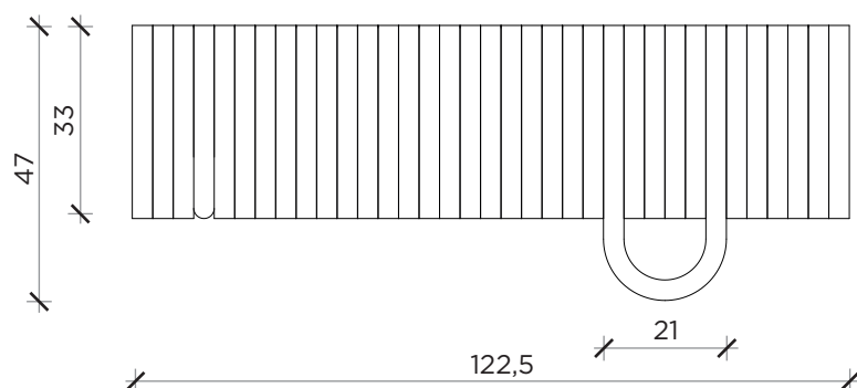
FRONTE | FRONT
