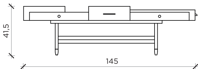
FRONTE | FRONT
