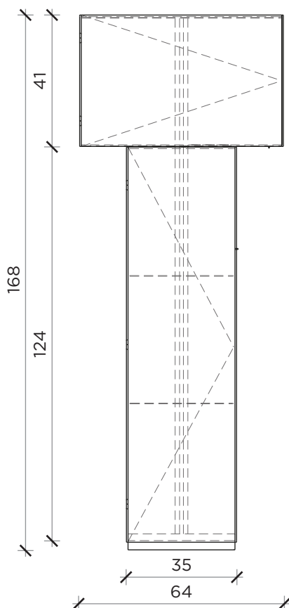
FRONTE | FRONT
