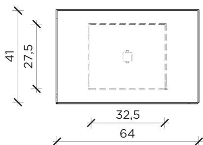
FRONTE | FRONT
