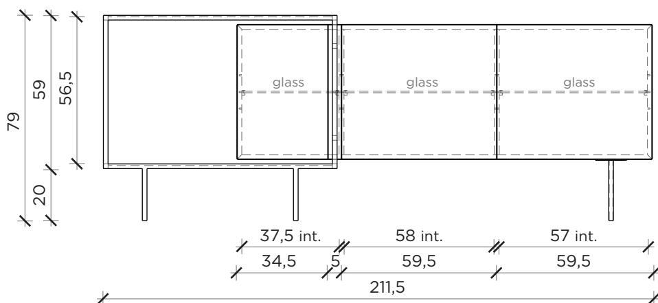
FRONTE | FRONT
