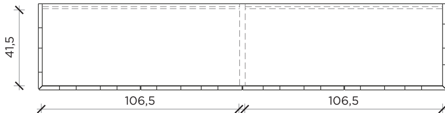
FRONTE | FRONT
