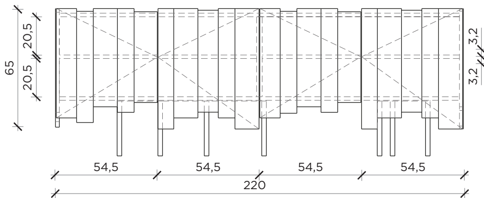
FRONTE | FRONT
