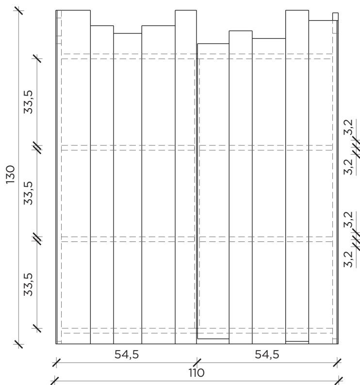
FRONTE | FRONT
