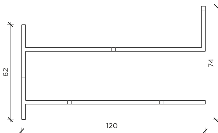
FRONTE | FRONT
