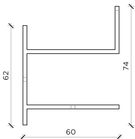
FRONTE | FRONT
