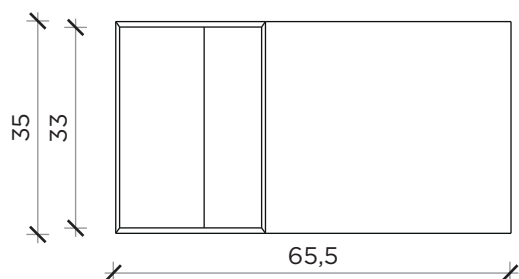
FRONTE | FRONT
