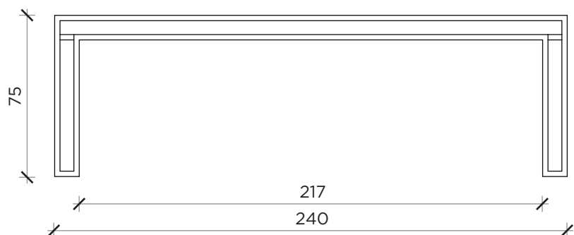
FRONTE | FRONT
