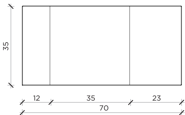
FRONTE | FRONT
